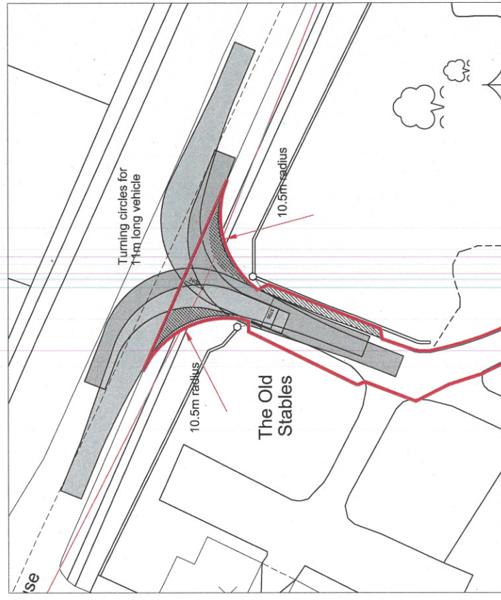
PROPOSED SITE PLAN WITH VEHICLE TRACKING (1:200)
